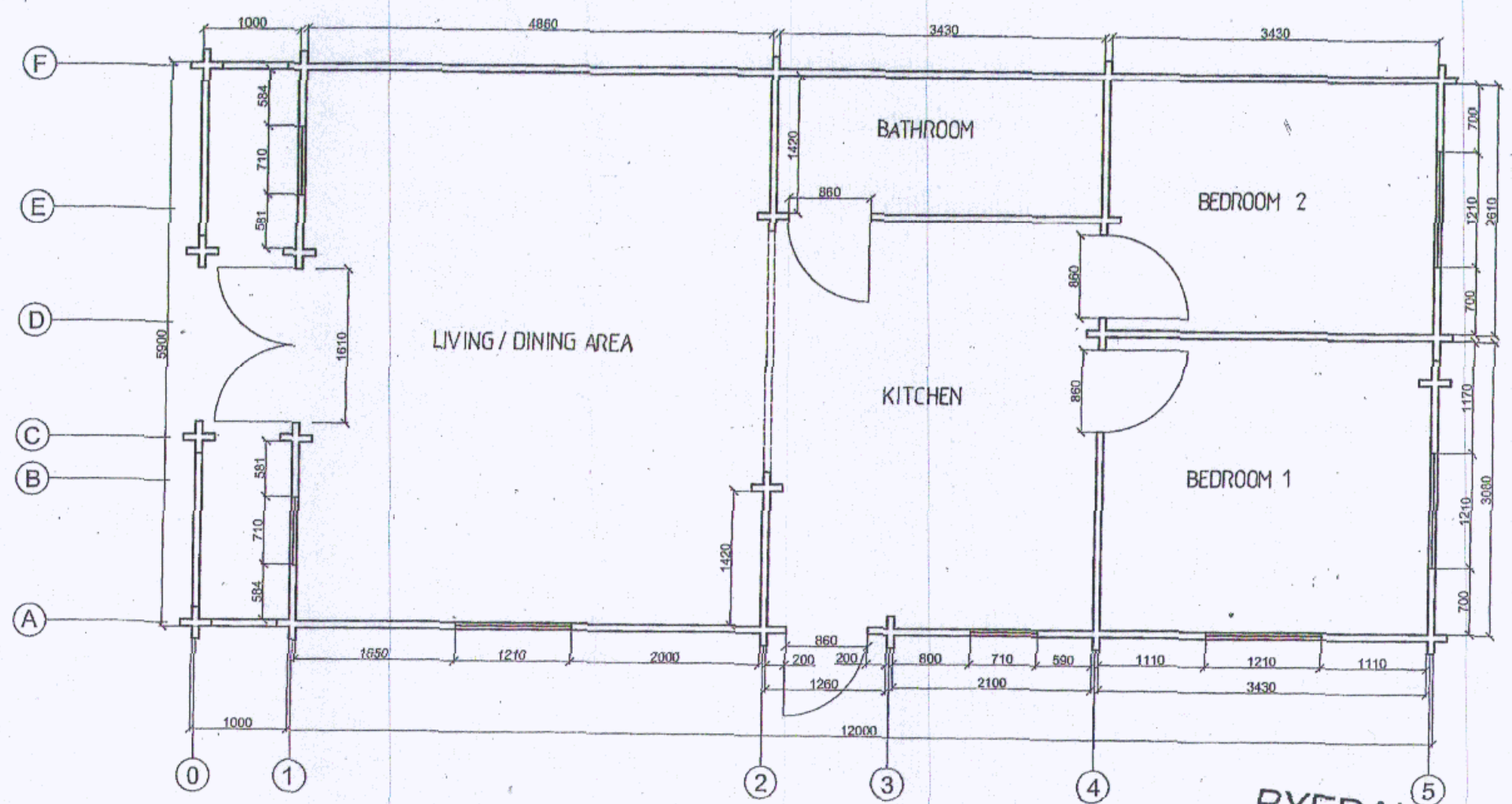
FLOOR PLAN
